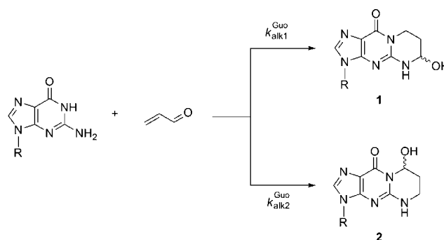
Scheme 4 Alkylation of guanosine by acrolein.
