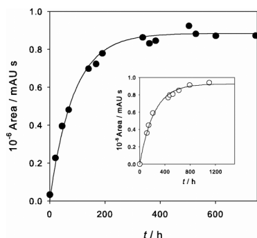
Fig. 7 Formation of the Guo-AN adduct (●): [Guo] 0 = 10 -4 M; [AN] 0 = 0.05 M and Guo-AM adduct (○): [Guo] 0 = 10 -4 M; [AM] 0 = 0.1 M. Variation in peak area with time. pH = 9.6; T = 37.5 °C.
